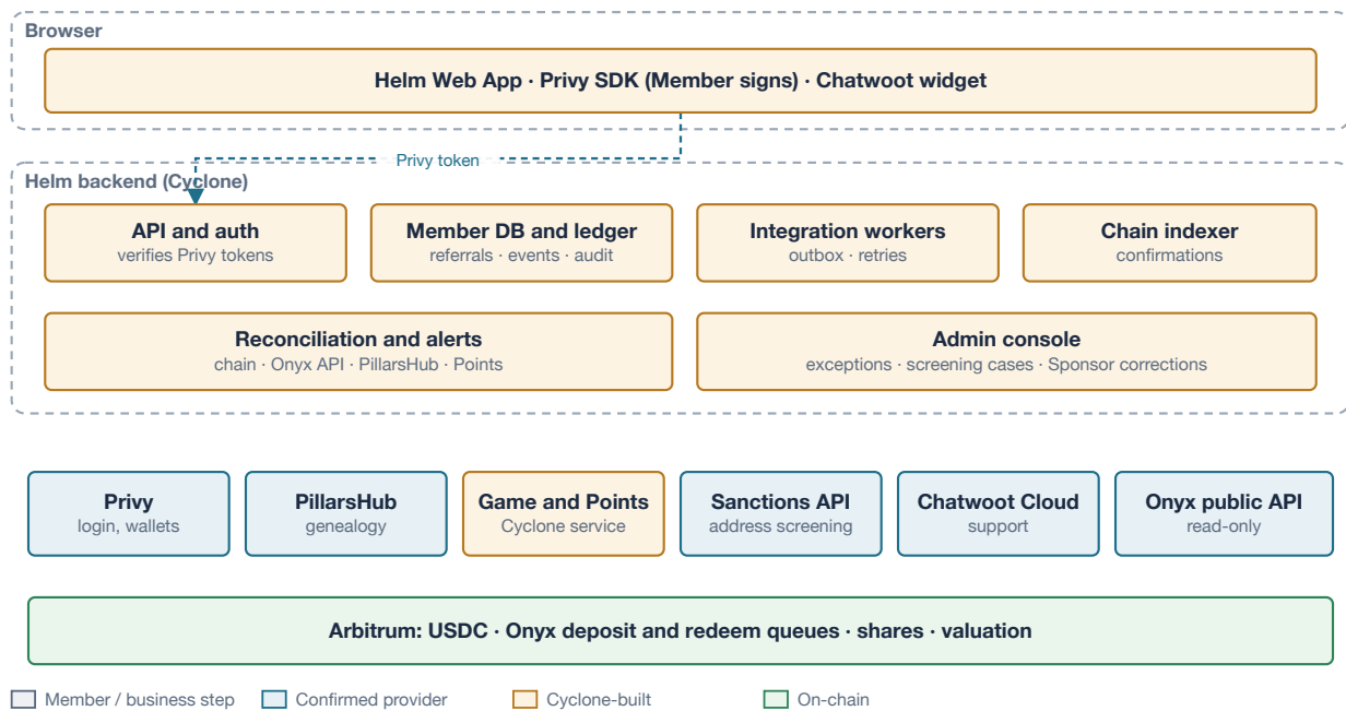
Figure 3: Technical architecture and trust boundaries.
