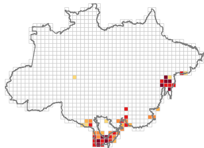
Z_{2047}^i (%), b=15
