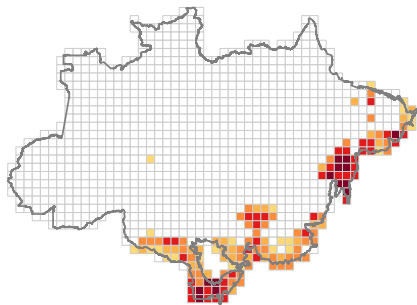
Z_{2037}^i (%), b=15
