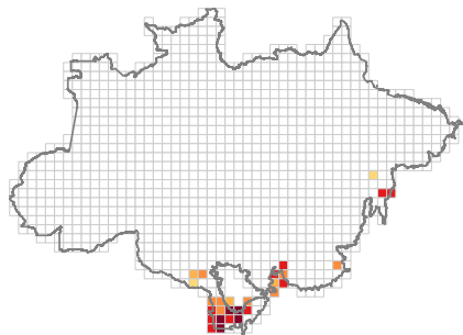
Z_{2032}^i (%), b=15
