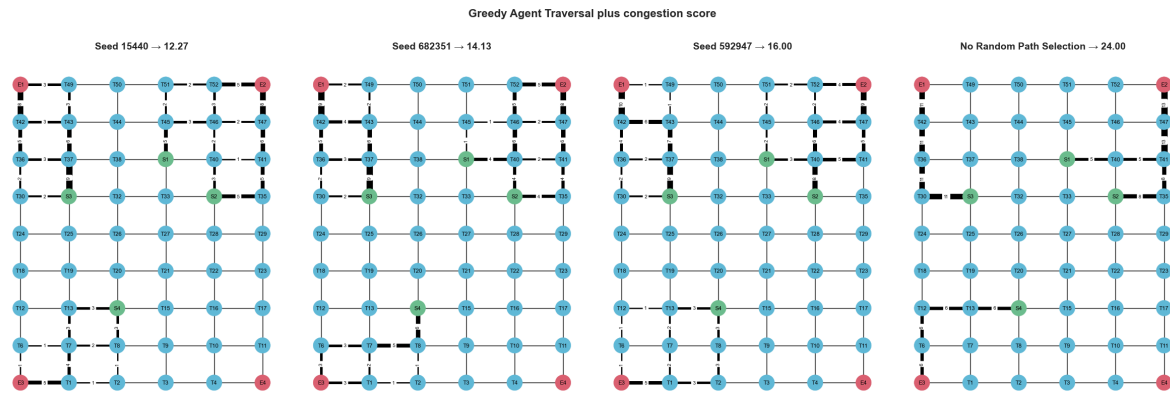
Figure 4.4: Greedy shortest path routing options across 3 seeds (from left) and first path selection (right). The thicker the edge weight in the figure show the frequency of use which varies across the seeds
