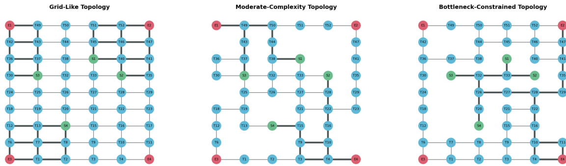
Figure 4.2: Network topologies from left to right; grid-like, moderate-complexity and bottleneck-constrained. The green nodes represent starting positions (S) and red exit positions (E).
