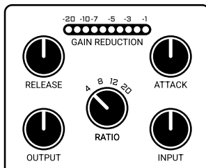
Figure 3. Basic compression settings
