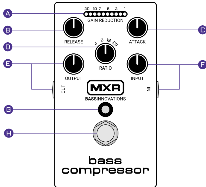
Figure 1. M87 Bass Compressor controls
