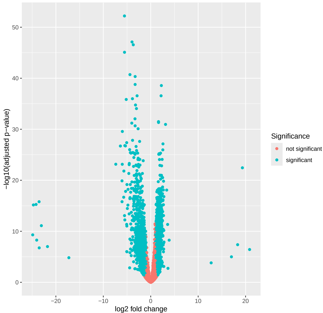
Volcano plot of Gene Expression (I vs E)
