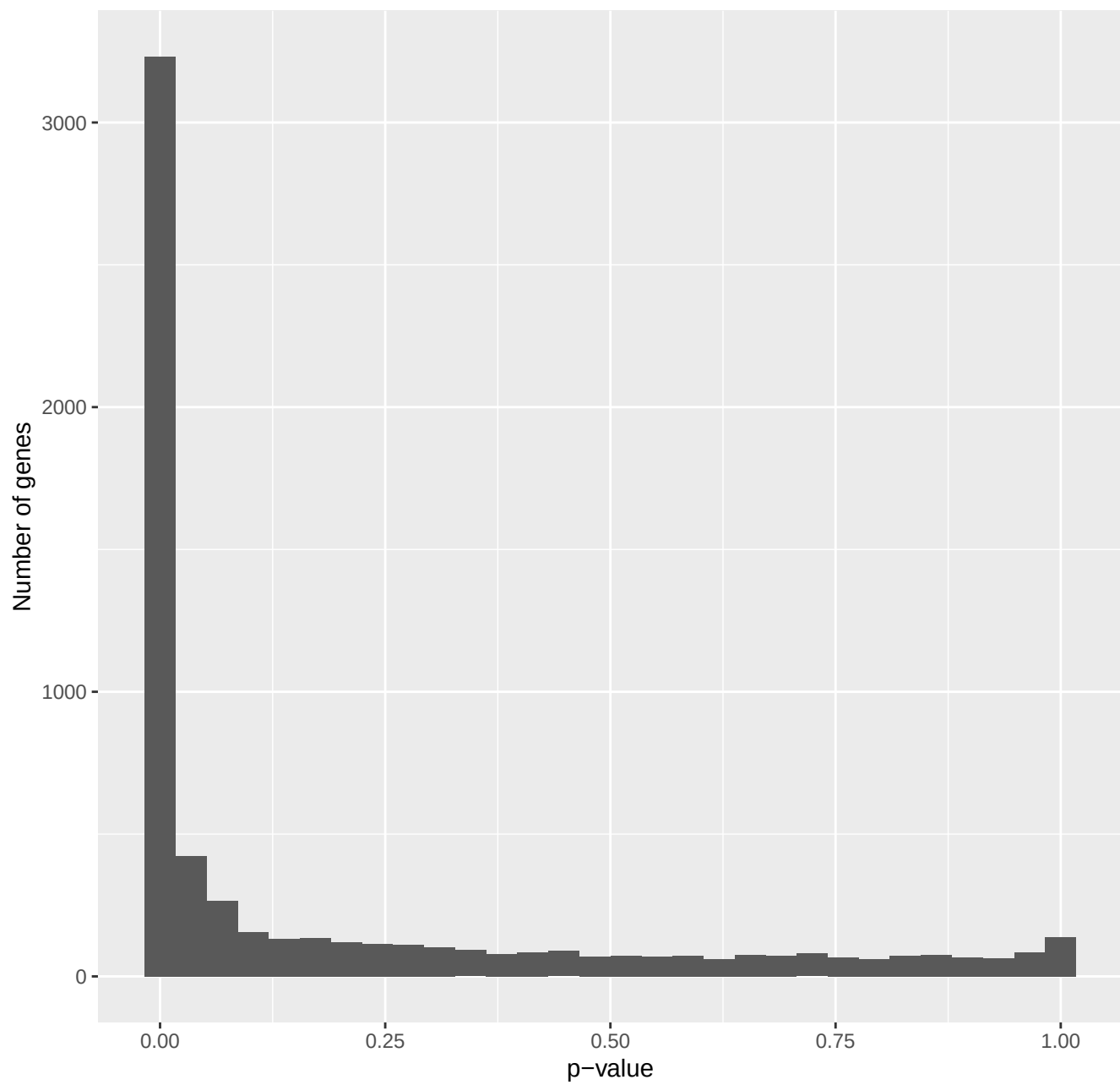
Distribution of P-values(I vs E)
