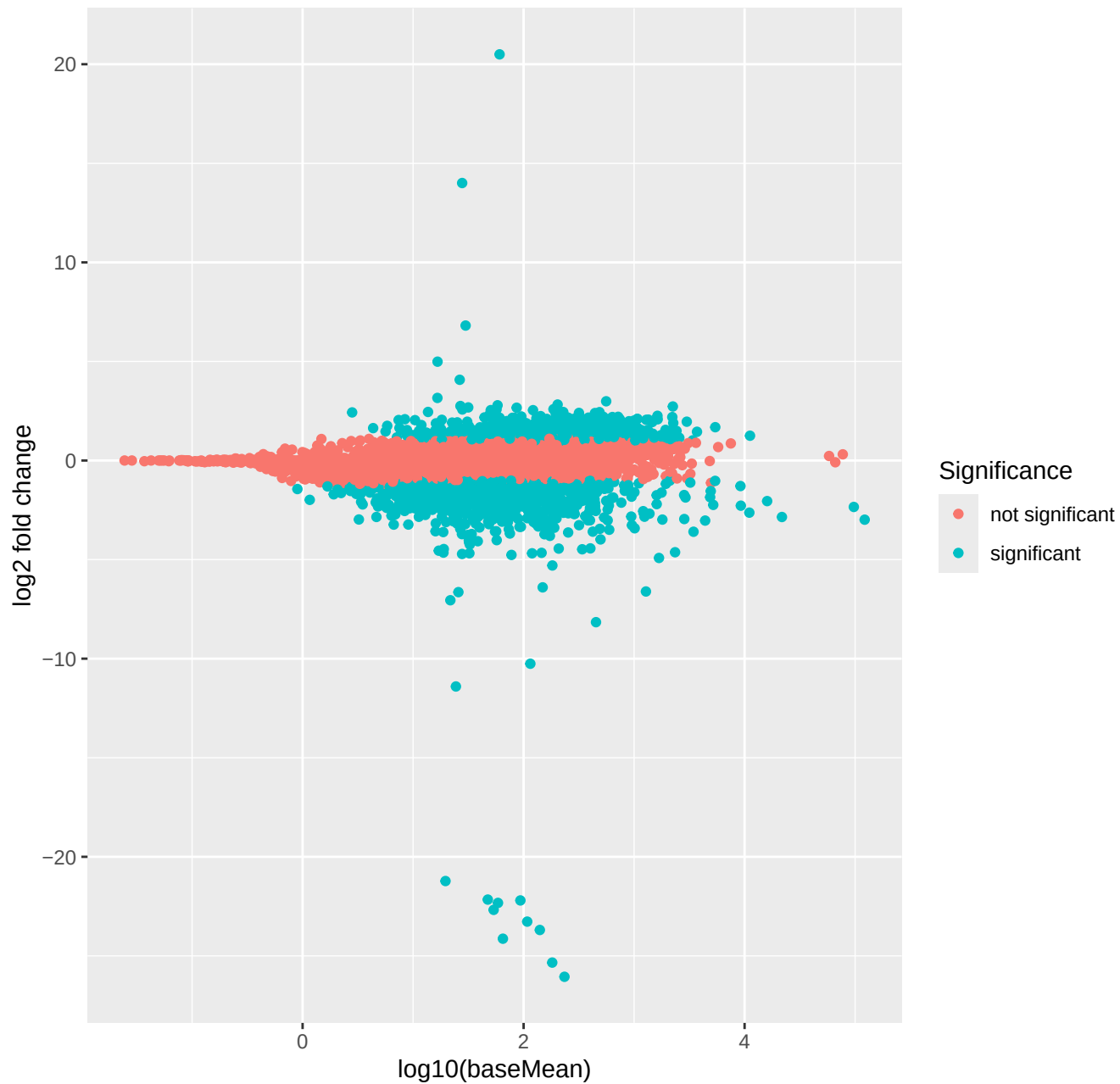
MA plot of Log2 Fold Change vs Mean Expression (G vs D)
