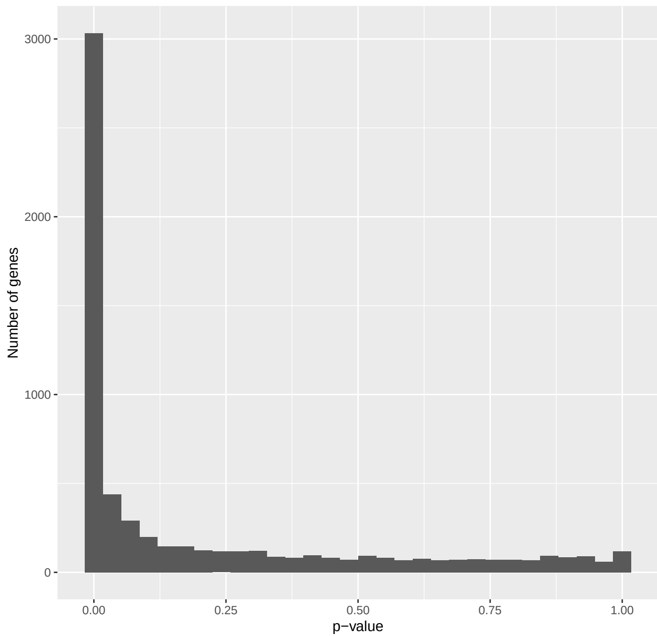
Distribution of p-values (G vs D)
