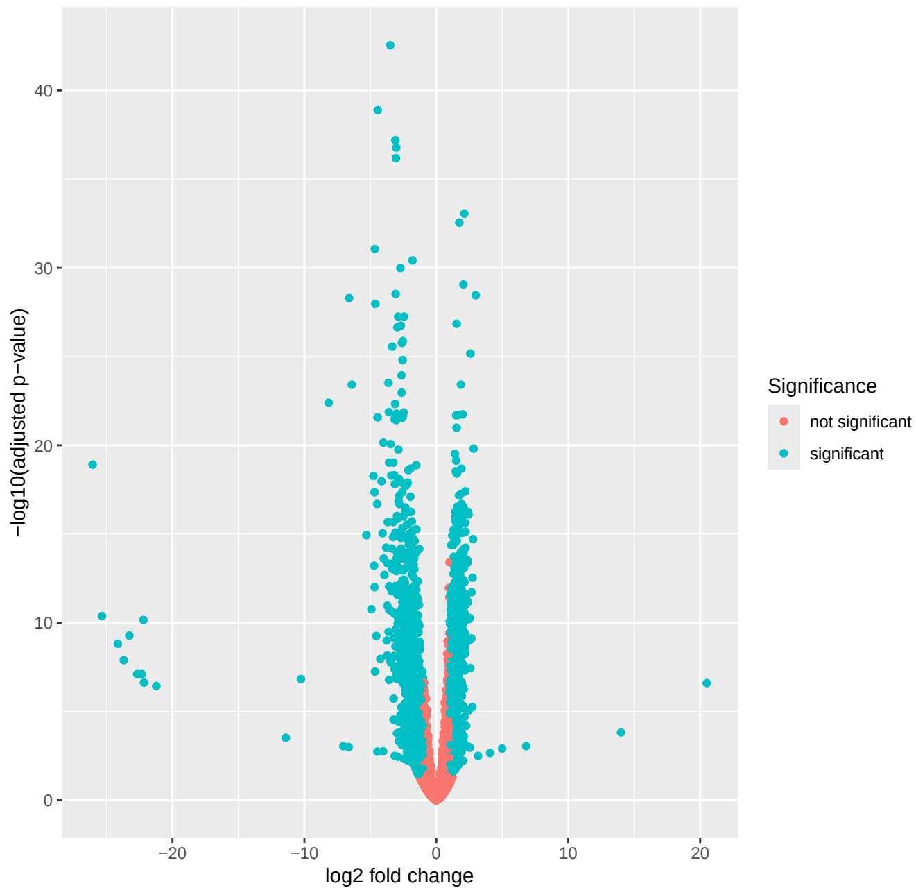
Volcano plot of Gene Expression (G vs D)
