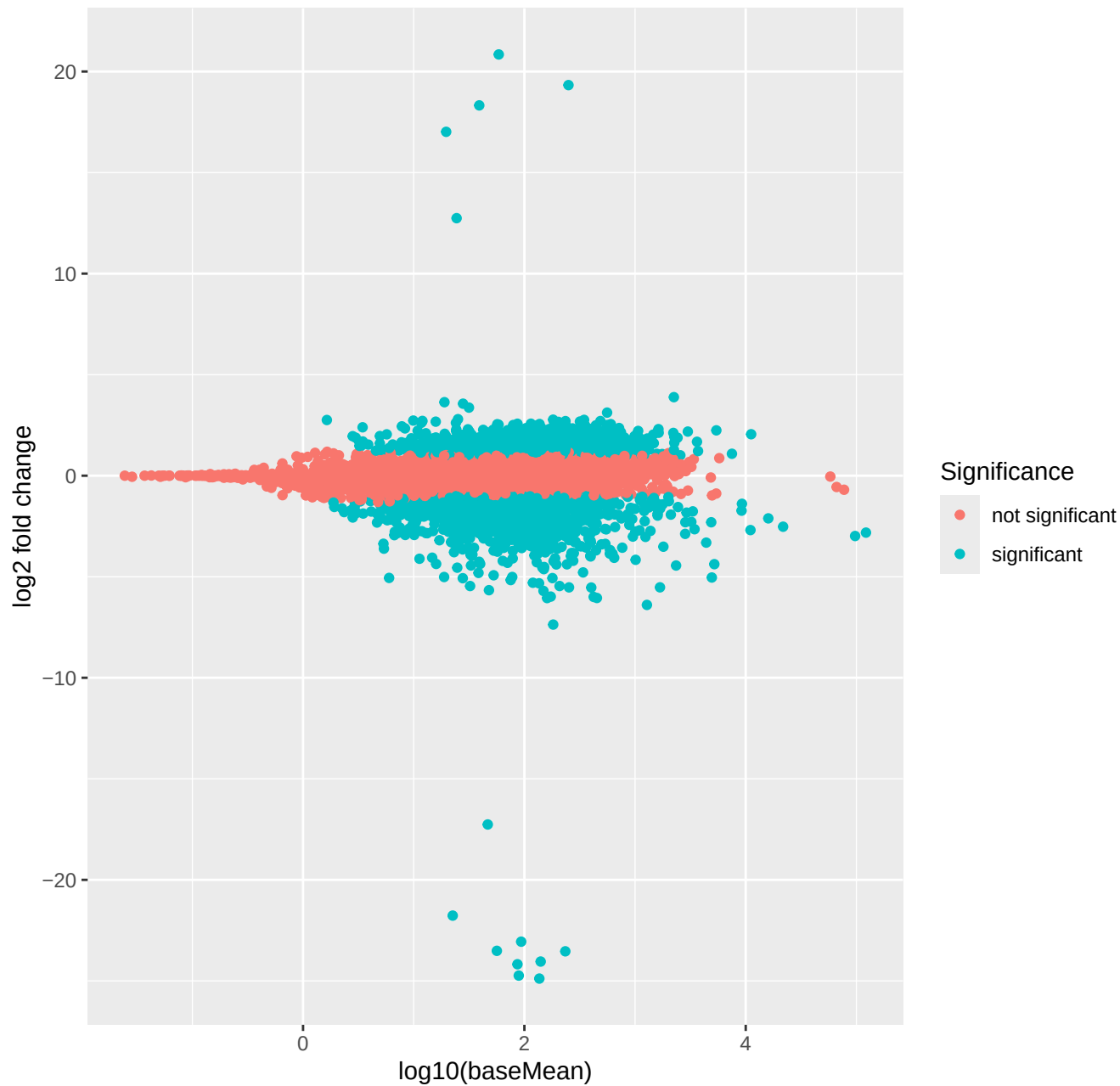
MA plot of Log2 Fold Change vs Mean Expression (I vs E)
