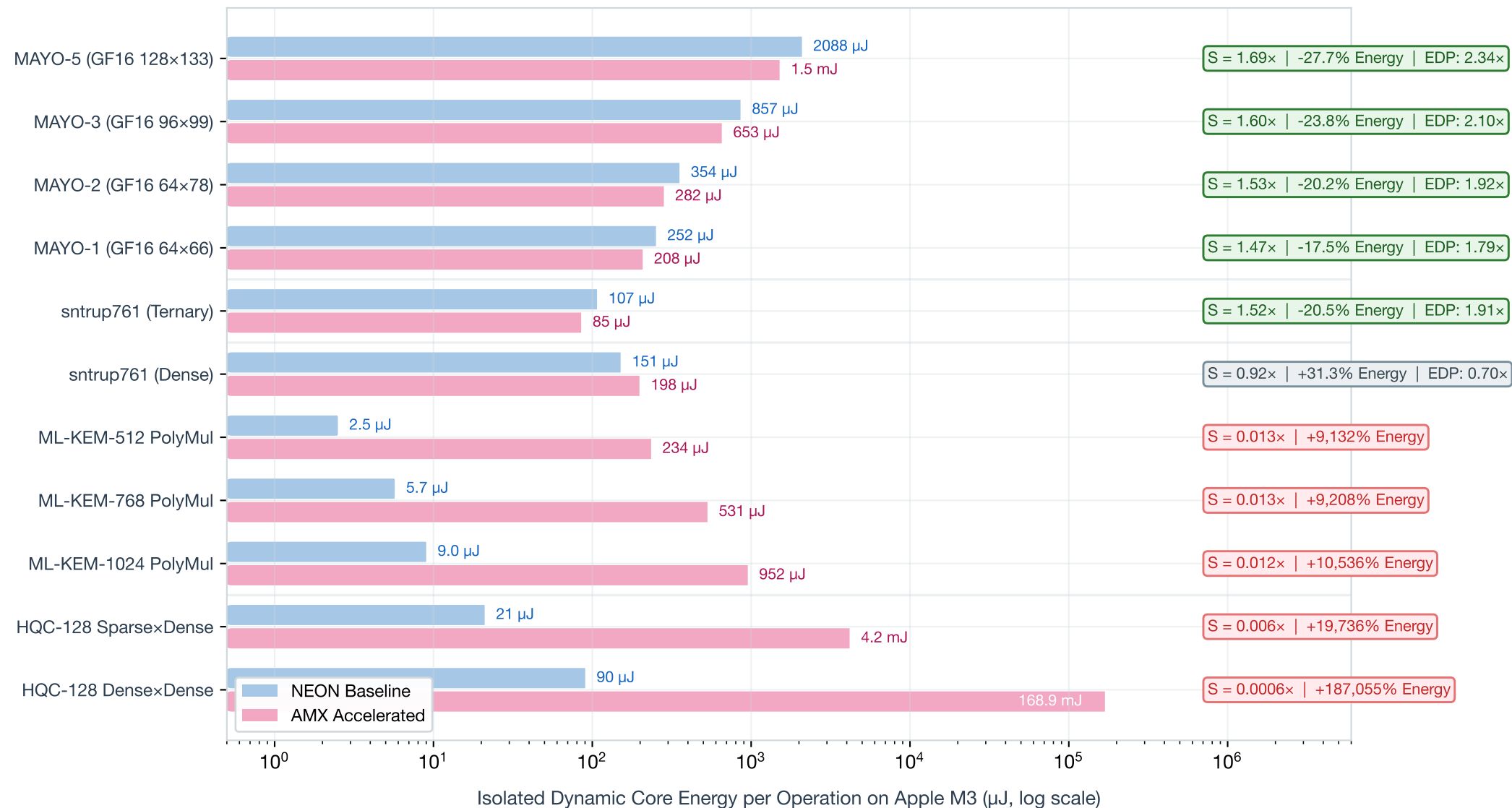
Cross-Scheme Active Energy per Operation on Apple M3: NEON Baseline vs. AMX Coprocessor
