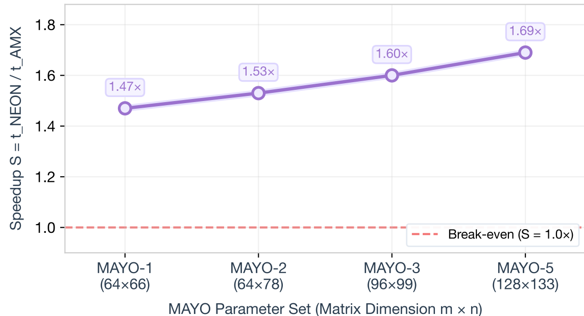
MAYO: Speedup Scales with Matrix Size on Apple M3
