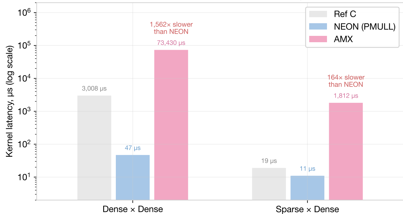
HQC-128: NEON PMULL vs AMX Kernel Latency on Apple M3
