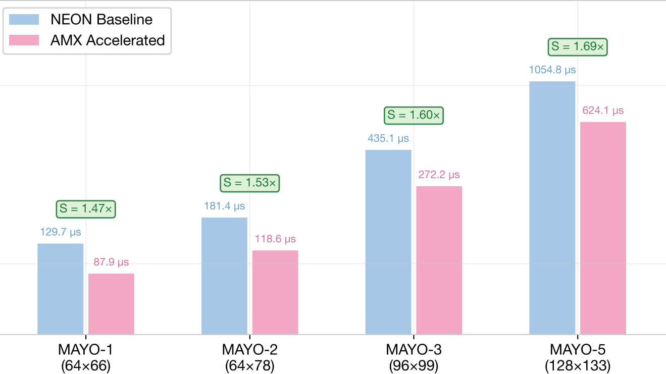
MAYO: NEON vs AMX Quadratic Form Latency on Apple M3
