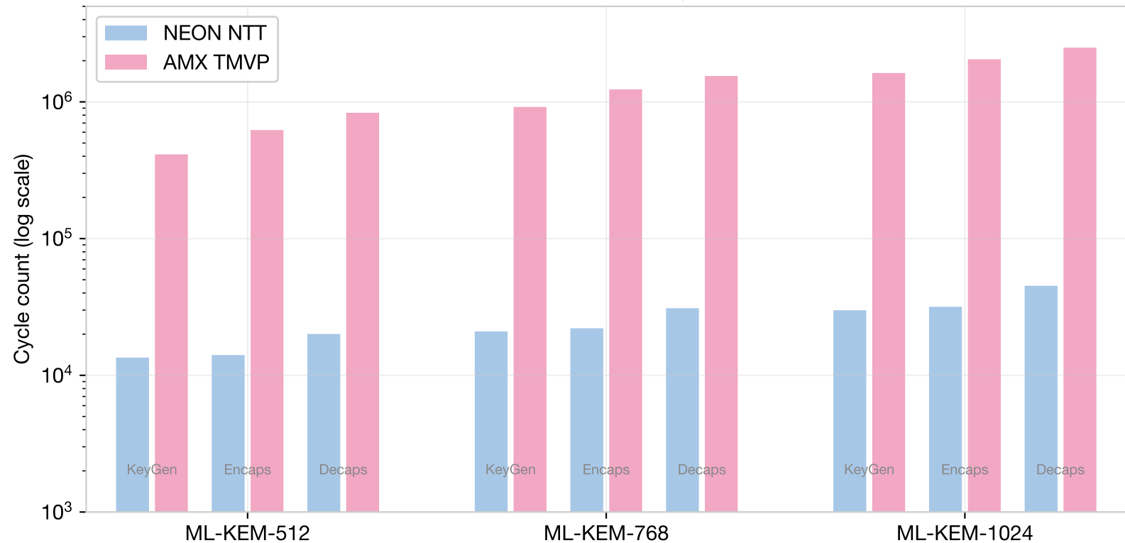
ML-KEM: NEON NTT vs AMX TMVP Cycle Counts on Apple M3
