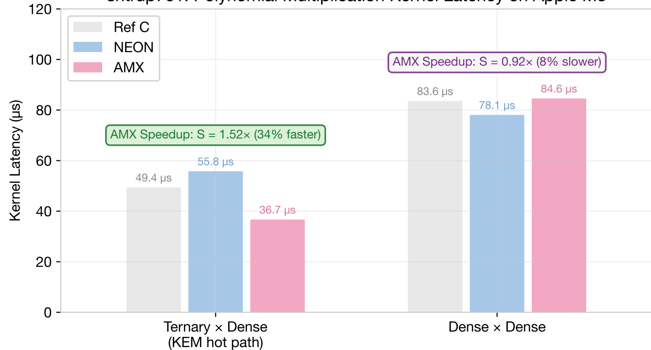
sntrup761: Polynomial Multiplication Kernel Latency on Apple M3
