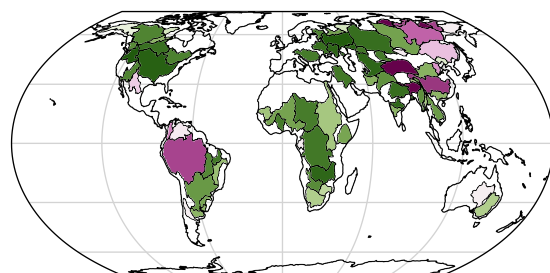
CSR GRACE/FO
