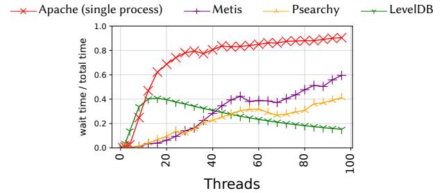
Figure 1. Ratio of time wasted waiting for the mmap_lock to total execution time on Linux 6.8.0 for various applications.
