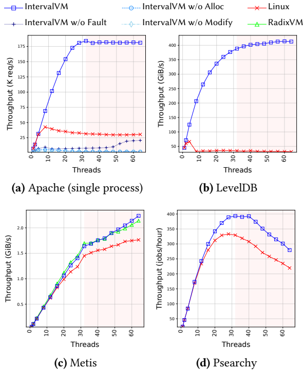
Figure 22. Multithreaded throughput of Apache (single process), LevelDB, Metis, and Psearchy.
