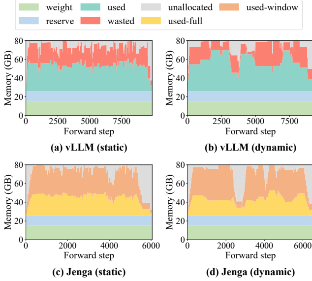
Figure 17. Timeline of memory usage for Ministral model. vLLM shows significant wasted memory due to memory fragmentation (in red), while JENGA minimizes waste.
