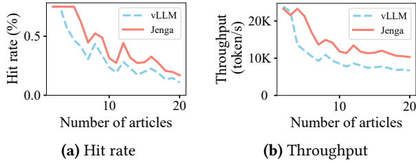
Figure 18. Prefix caching with different number of articles
