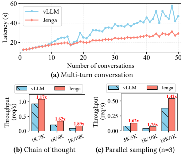
Figure 21. Typical workloads with Gemma-3 model. nK/mK means nK input tokens and mK output tokens
