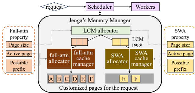
Figure 7. Overview of JENGA
