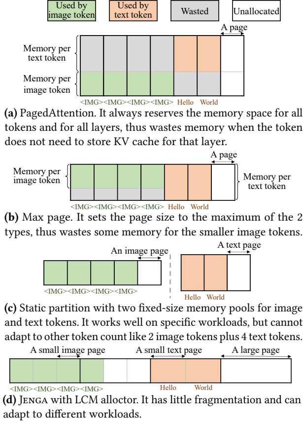
Figure 5. Different memory allocation strategies for Llama 3.2 vision model. Assume the KV cache size per token of text tokens is 1.5× that of image tokens.
