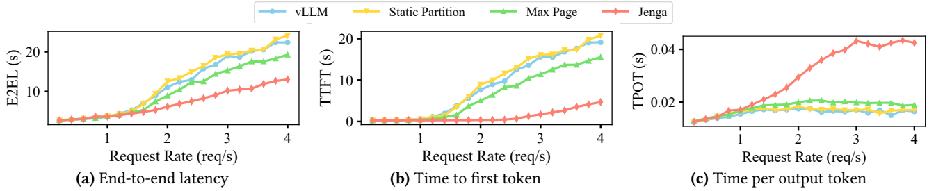
Figure 15. Averaged Latency for the Llama Vision Model with changing request rates
