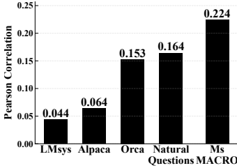
Figure 7. Pearson correlation (€ [-1, 1]) between example similarity and its helpfulness is weak.
