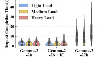
Figure 20. IC-Cache improves serving efficiency across serving loads.
