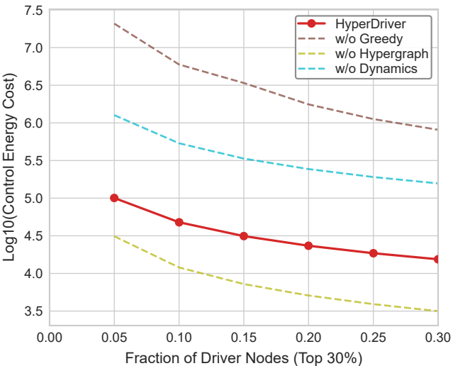
Ablation: Babu
