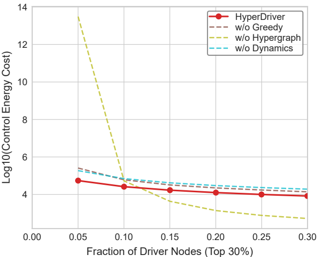
Ablation: Ito
