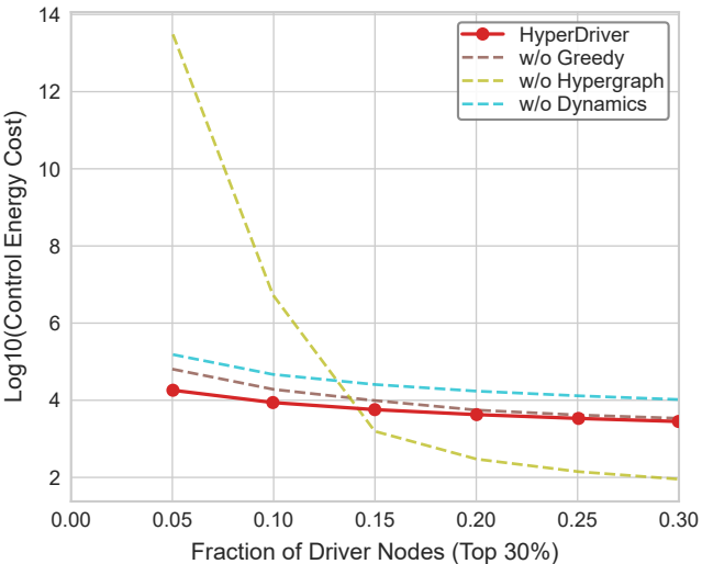
Ablation: Tarassov
