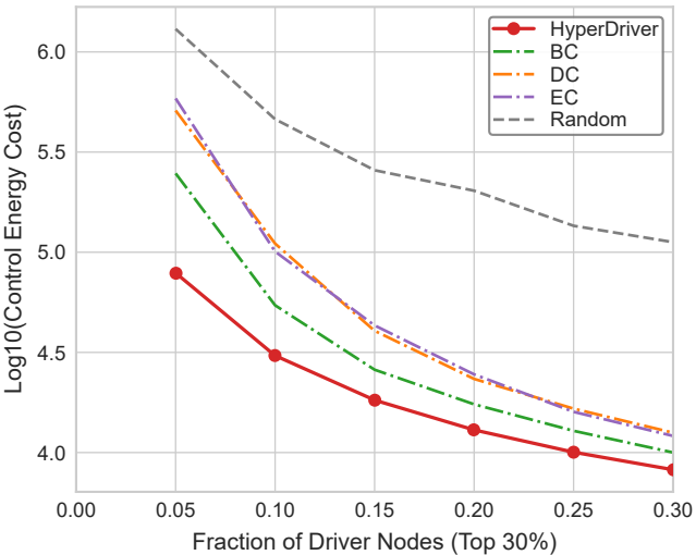
Efficiency: Krogan_LCMS
