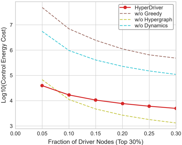
Ablation: Ho
