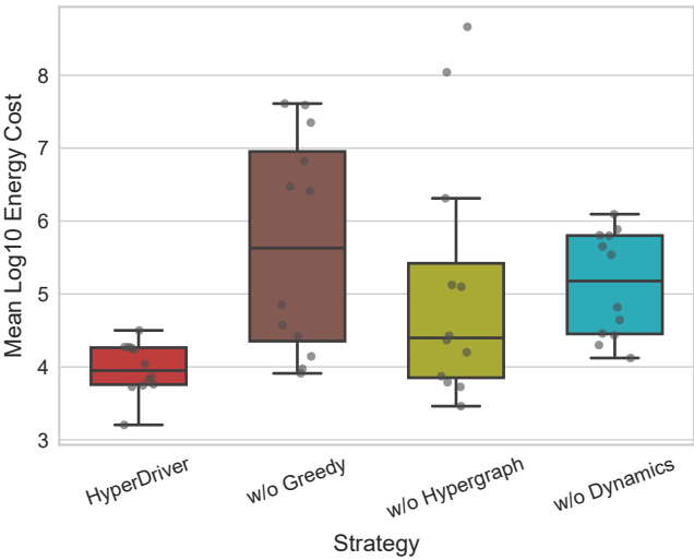
Global Ablation Summary
