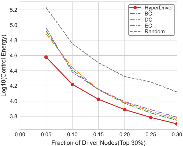
Control Energy(Ho)
