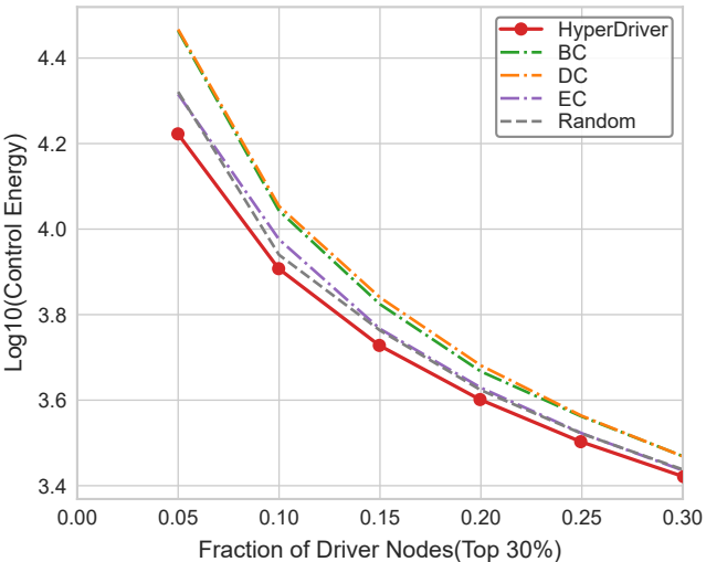
Control Energy(Uetz)
