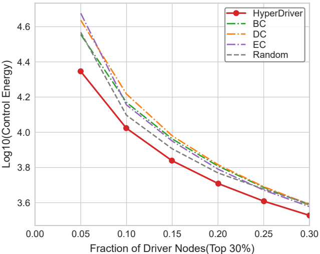
Control Energy(Yu)
