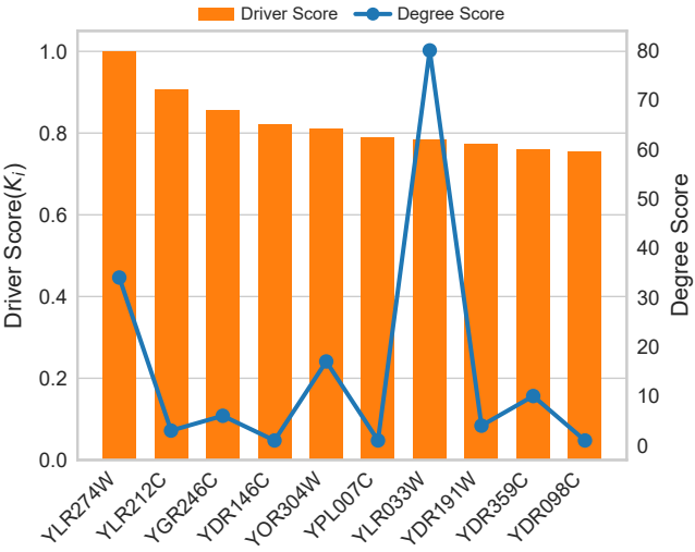
Top10 Drivers(Lambert)
