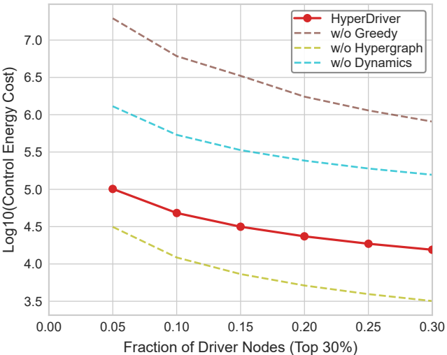
Ablation: Babu
