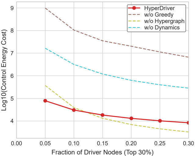
Ablation: Gavin
