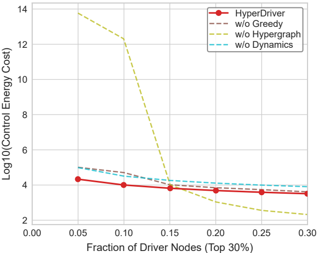
Ablation: Yu
