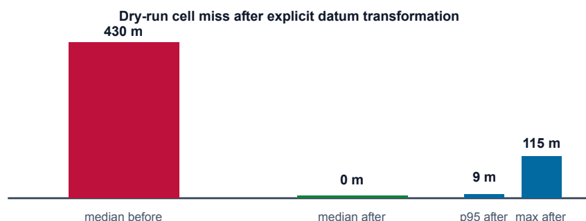
Figure 5 — cell miss in the all-437-sheet dry run: the median collapses from 430 m to 0 m.
