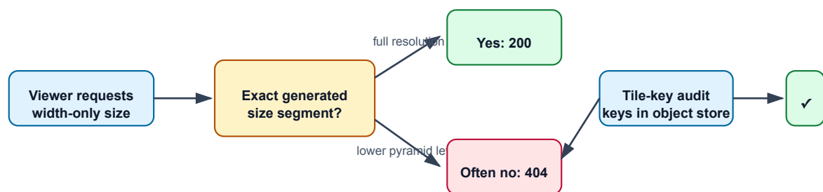
Figure 6 — a request can be valid IIIF syntax and still miss the server’s tile grid.
