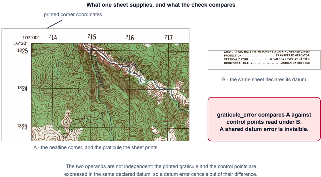
Figure 4: The source of the shared assumption. The graticule and the control points are interpreted in the sheet’s declared datum. Their agreement can test internal consistency but cannot independently establish that datum. This correctly placed sheet illustrates the inputs, not an example of the measured displacement. A Lưới 6441-4, AMS Series L7014 (US Army Map Service; scan by the Perry-Castañeda Library, University of Texas at Austin). US Government work, public domain.
