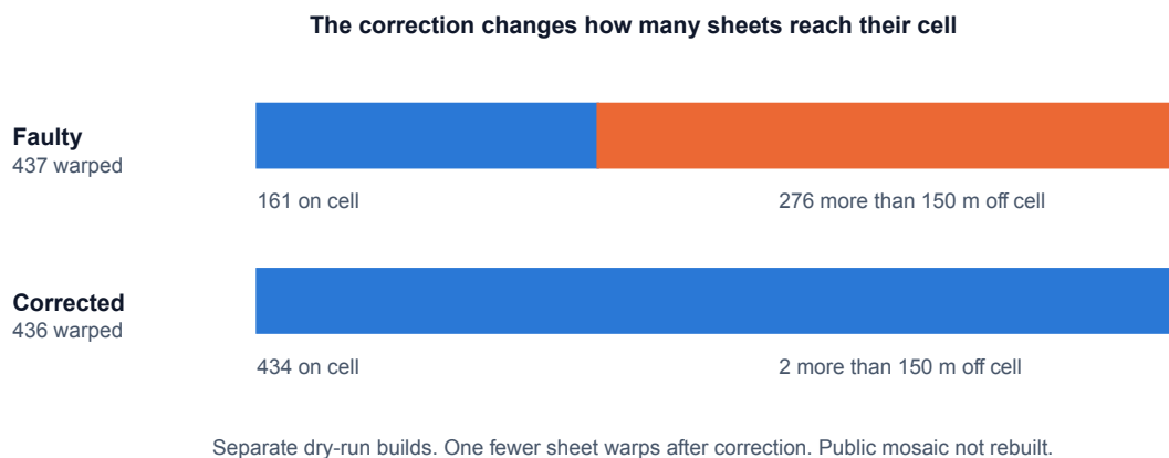
Figure 7: The correction recovers cell placement in the local reproduction. Bars use a common sheet-count scale. The faulty build places 161 of 437 sheets on cell; the corrected build places 434 of 436. Orange marks sheets more than 150 m off cell. The two remaining failures require review. These results do not measure a rebuilt public mosaic.
