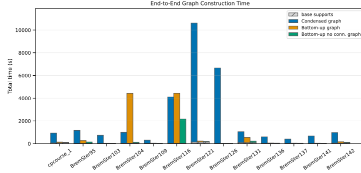
Fig. 6. End-to-end runtime comparison, in seconds, between Condensed, connected Bottom-up, and Bottom-up no-connectivity constructions on the thirteen benchmark instances. Stacked bars separate the common base-support computation from the approach-specific graph-construction phase.
