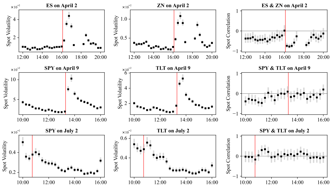
Figure 8: The figure shows the intraday patterns of spot volatility and spot correlation on three distinct dates of the 2025 tariff cycle. Each row corresponds to one event day. The first two columns report the estimated spot volatilities. The third column reports the estimated spot correlation. Gray bands represent 95% confidence intervals. The vertical lines mark the exact times of the posts.
