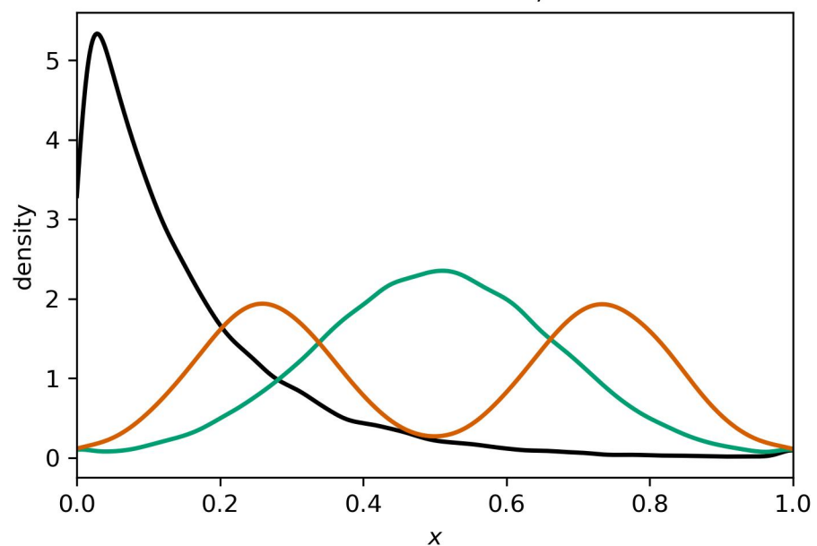
Covariate distributions, n = 500
