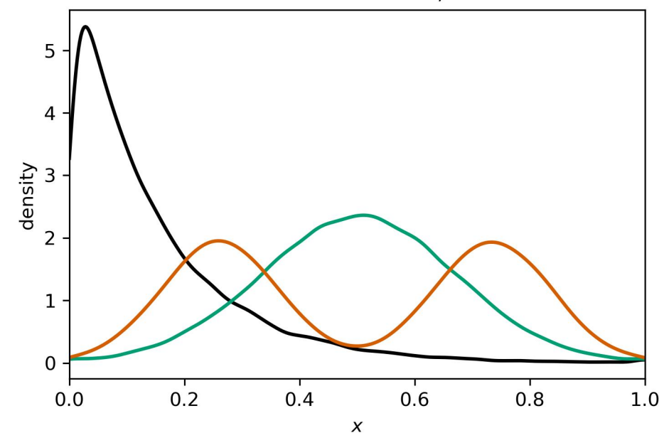
Covariate distributions, n = 500
