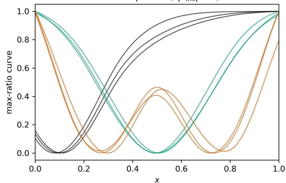
Distribution comparison, |\Gamma_{int}| = 5, n = 500
