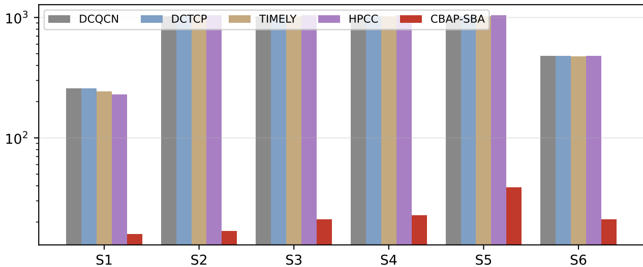
max queuing delay (us)
