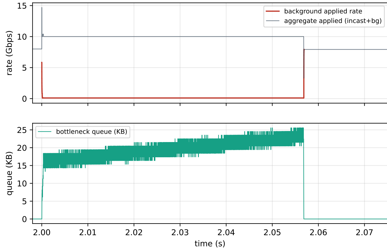
S3: capacity migration 8G->0.1G->8G and queue (CBAP-SBA, mx_s3_cbapsba)
