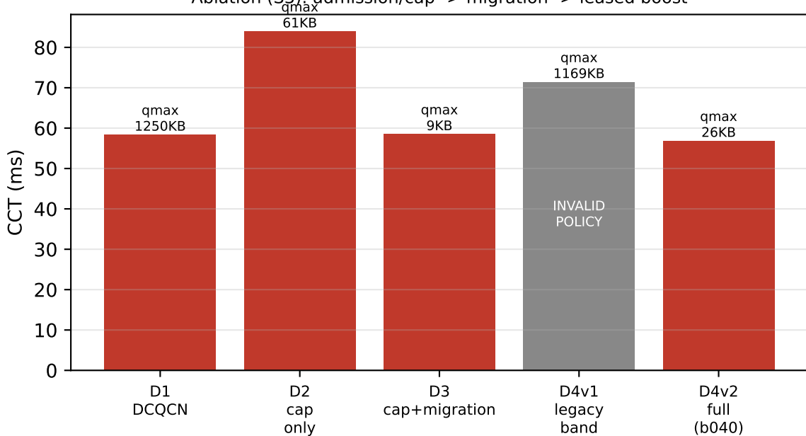
Ablation (S3): admission/cap -> migration -> leased boost
