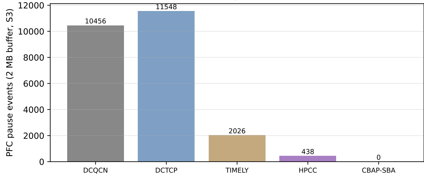
Shallow-buffer annex: PFC exposure (8 MB run had 0 for all)
