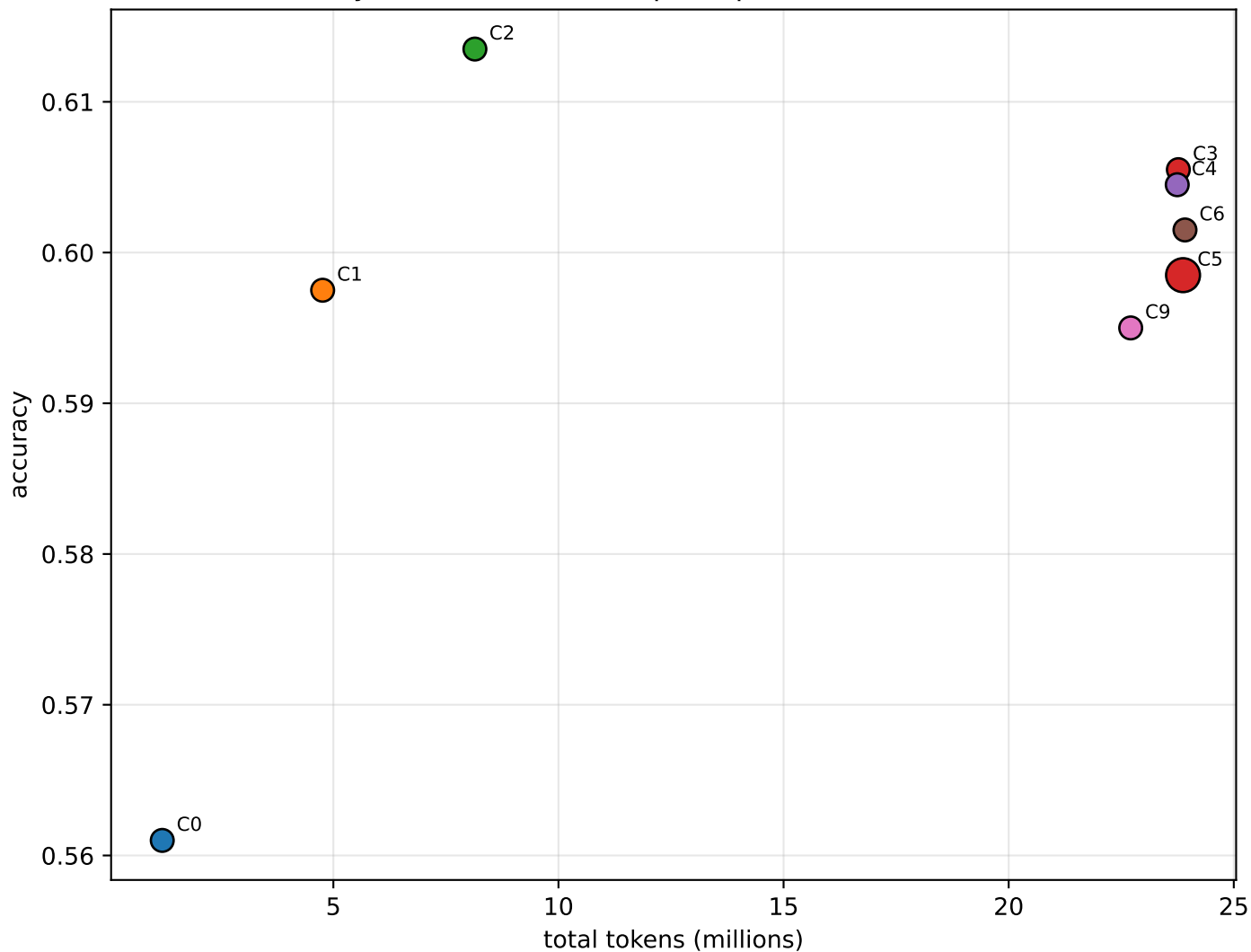
Accuracy vs token cost (one point per condition/benchmark)
