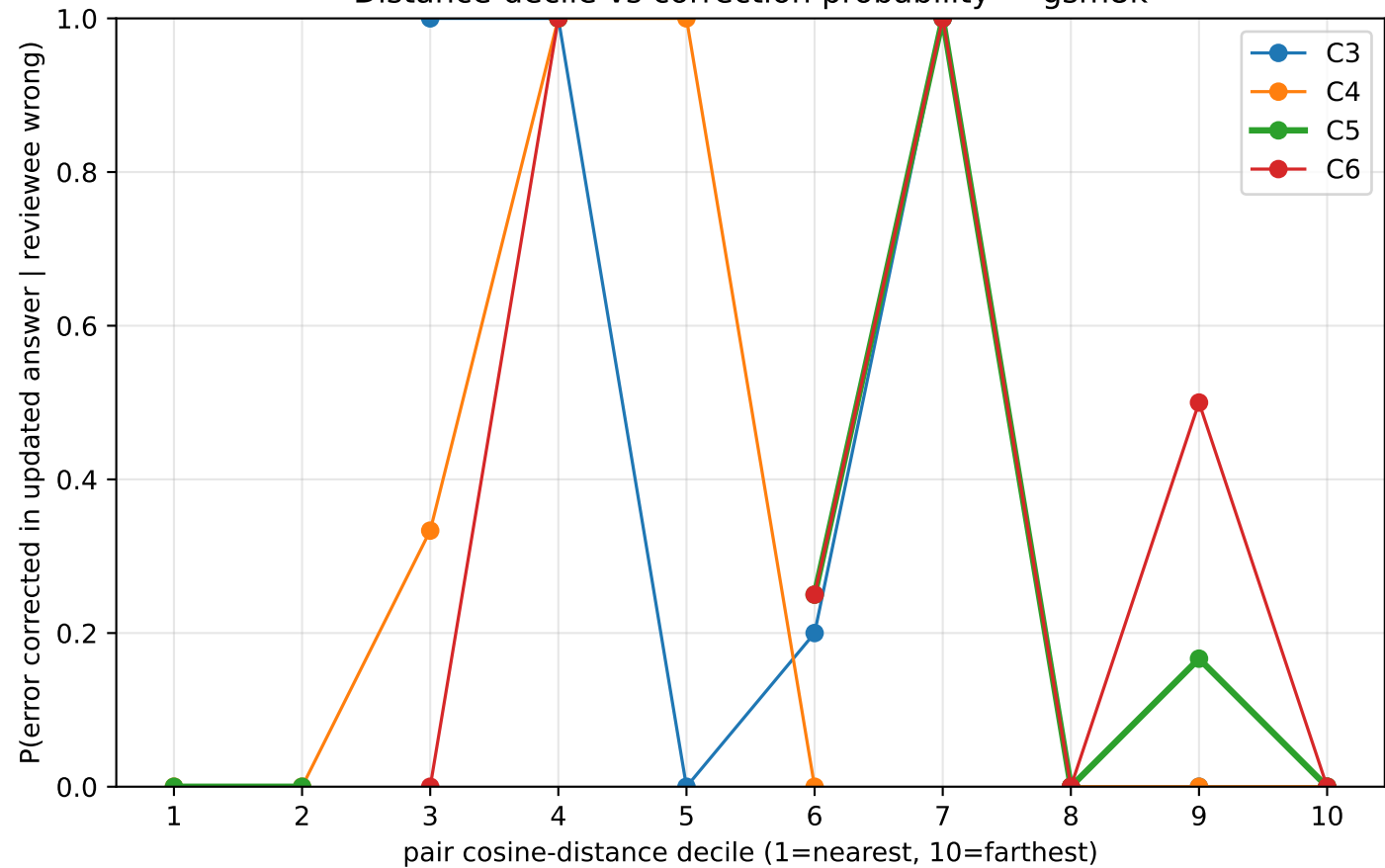
Distance-decile vs correction probability — gsm8k
