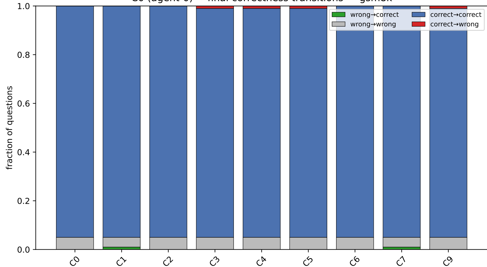
C0 (agent-0) → final correctness transitions — gsm8k
