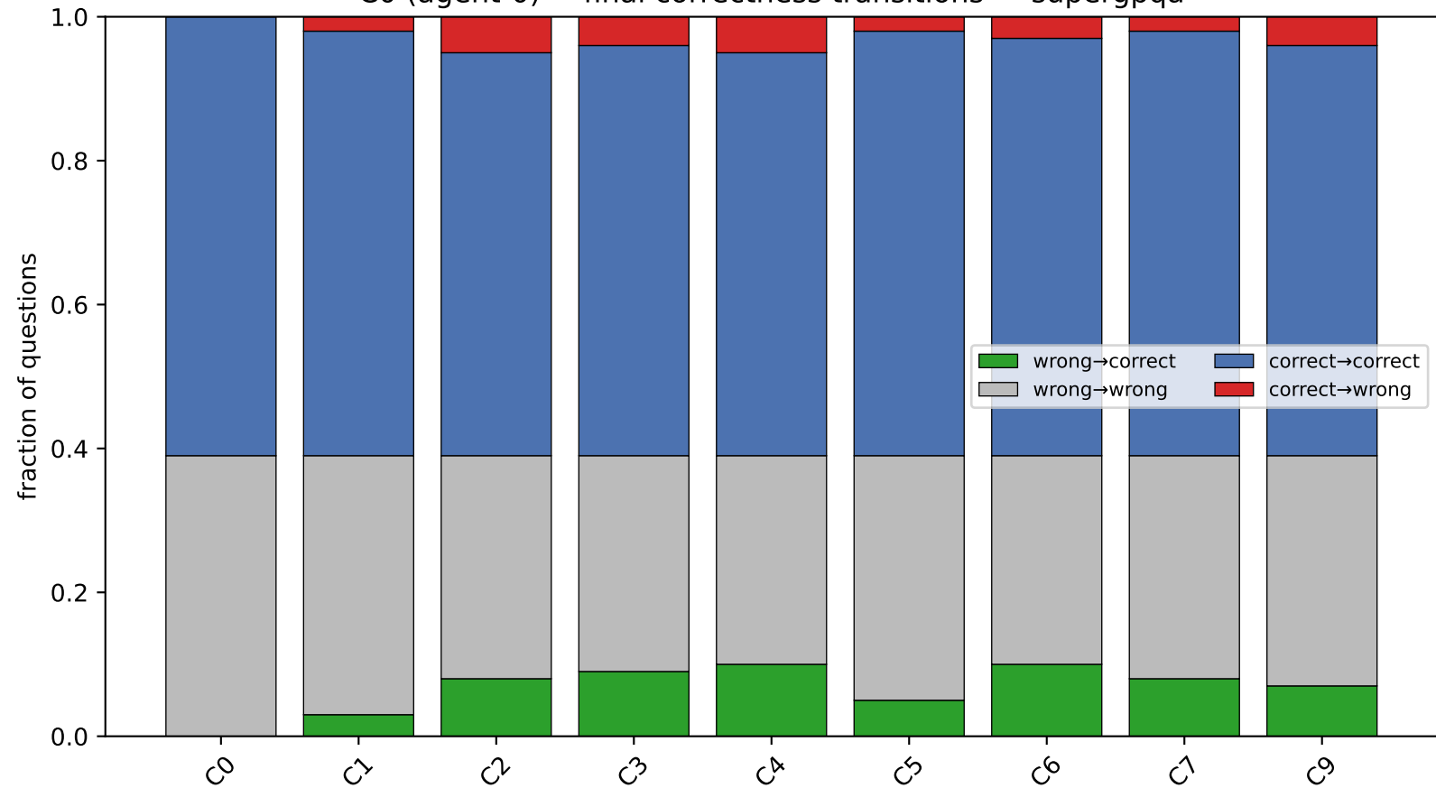
C0 (agent-0) → final correctness transitions — supergpqa
