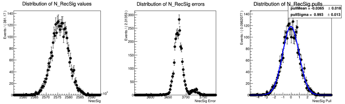
Figure (4.15) Plots showing distributions of the fitted signal yields, errors and the pull distribution of toy Monte Carlo pseudo-fits where the width of the Gaussian is floated.
