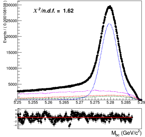
Figure (4.19) Total fit of tagged B mesons on Monte Carlo simulated data.
