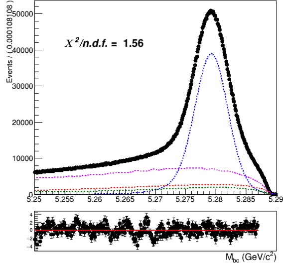
Figure (4.14) Total fit of tagged B mesons on Monte Carlo simulated data with sigma-Gauss free.
