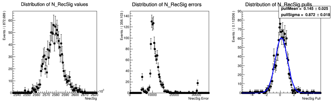
Figure (4.13) Plots showing distributions of the fitted signal yields, errors and the pull distribution of toy Monte Carlo pseudo-fits where the width of the Crystal Ball is floated.
