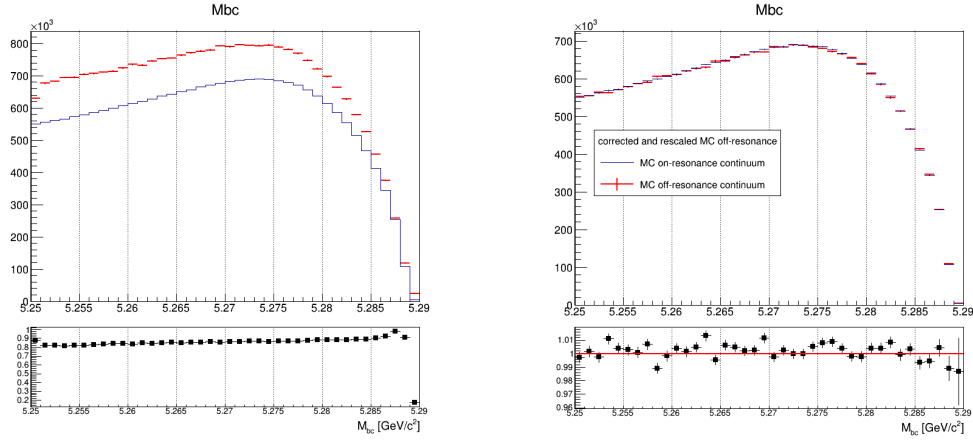
Figure (7.9) On the left: M_{bc} distributions of the MC off-resonance sample and the MC continuum sample. On the right: M_{bc} distributions of the corrected scaled MC off-resonance and on-resonance MC continuum.
