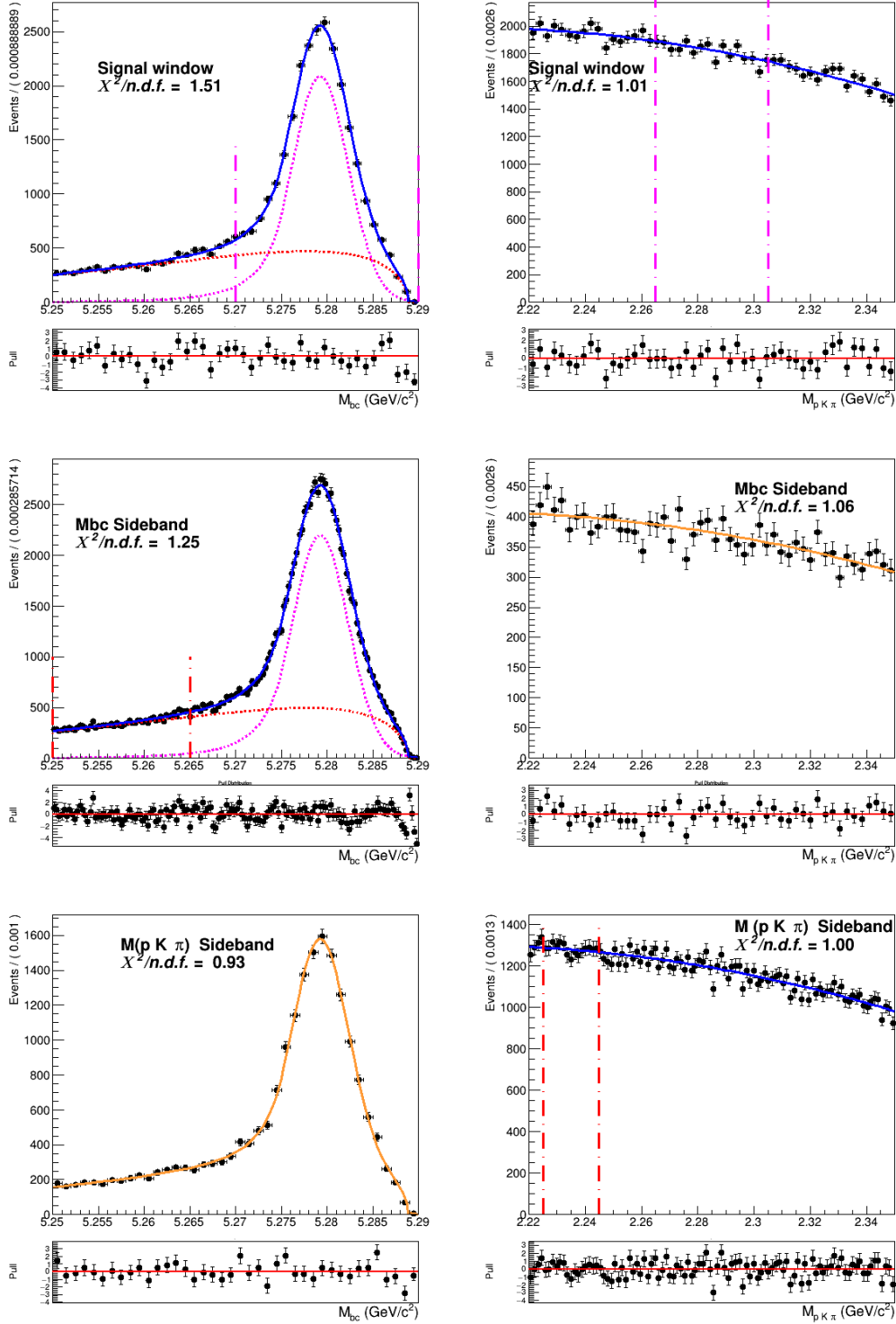
Figure (12) Signal region and sidebands of the two dimensional fit of generic background shown in ??
