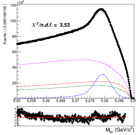
Figure (7.11) Total fit of tagged B^+ mesons candidates on data
