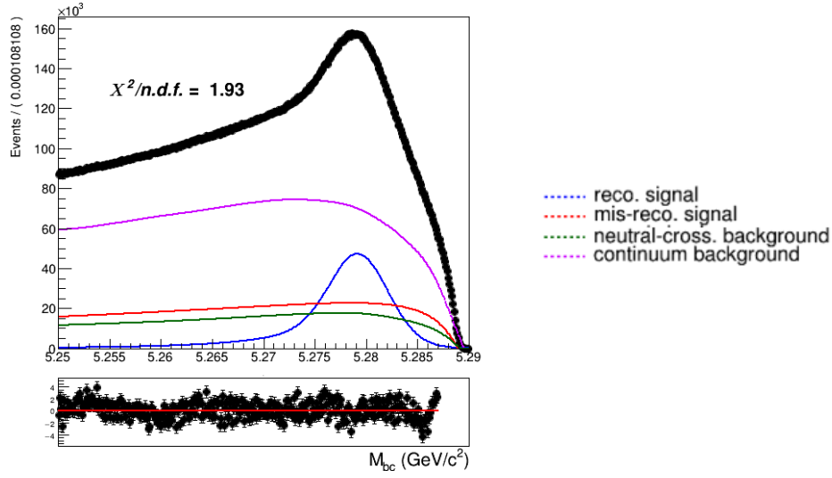
Figure (7.10) Total fit of tagged B mesons
