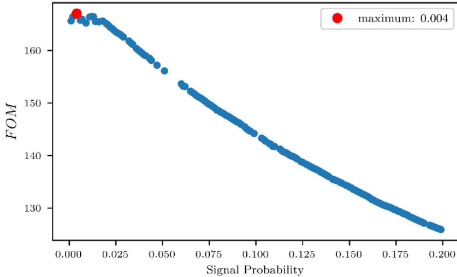
Figure (19) Figure of Merit values calculated at several cuts on the SignalProbability variable.
