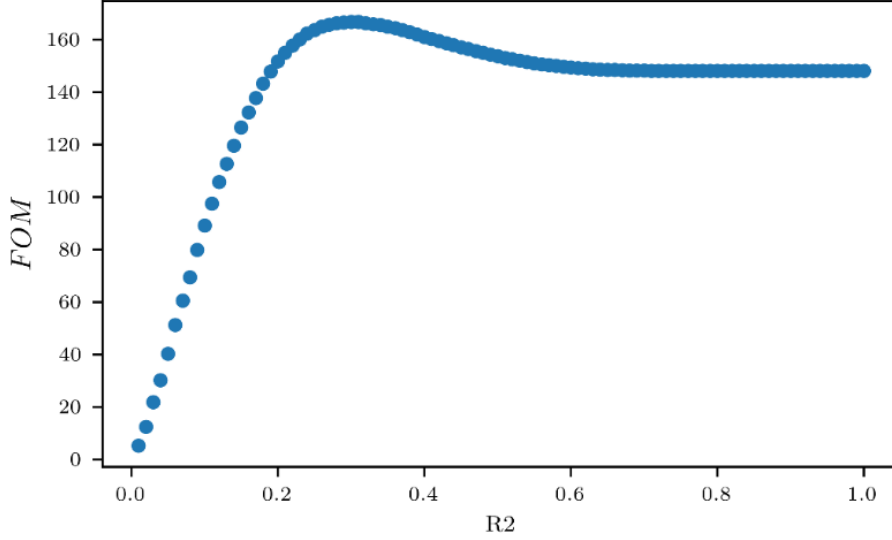
Figure (18) Figure of Merit values calculated at several cuts on the foxWolframR2 variable.
