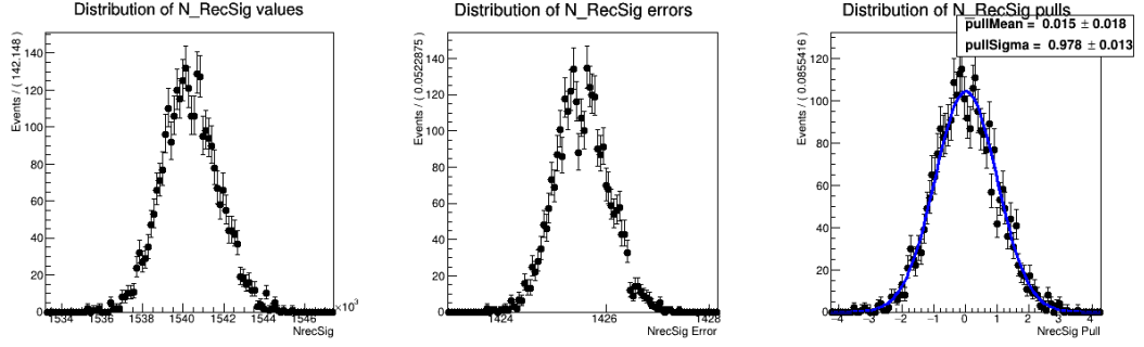
Figure (4.20) Plots showing distributions of the fitted signal yields, errors and the pull distribution of all pseudo-fits.
