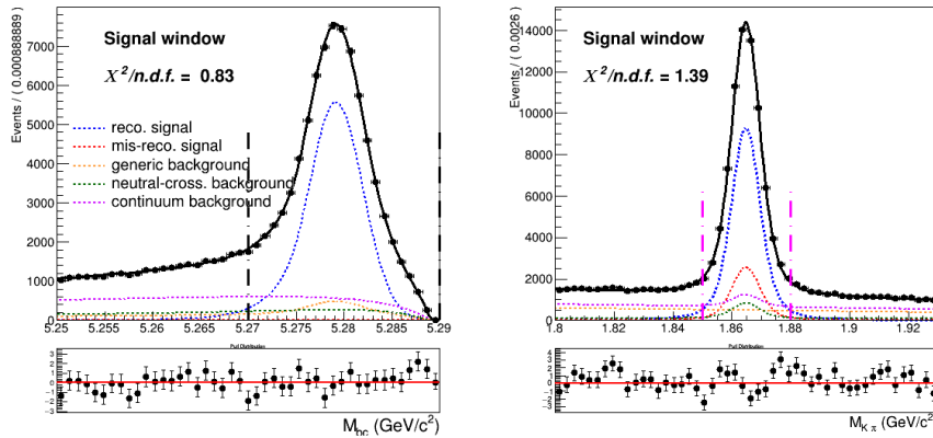
Figure (21) Signal region ( 1.85 < M(\pi K) < 1.88 \text{ GeV}/c^2 and 5.27 < M_{bc} < 5.29 \text{ GeV}/c^2 ) projections of the two dimensional fit on stream0 (Fig. 7.6).
