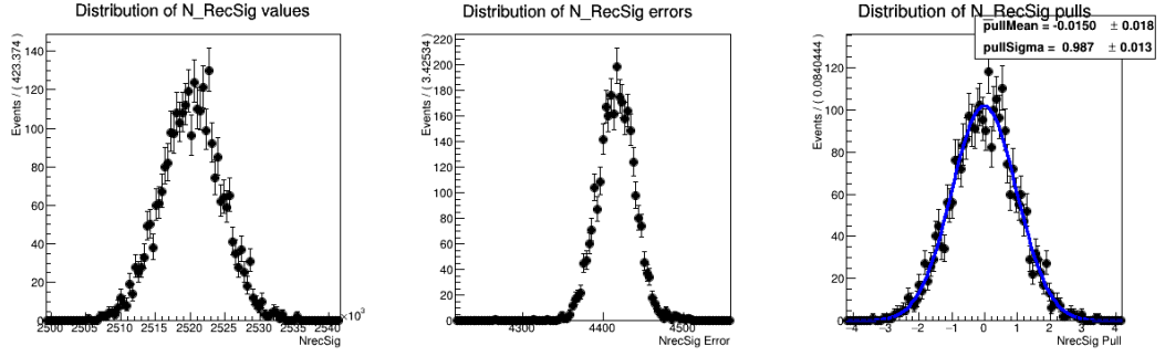
Figure (4.16) Plots showing distributions of the fitted signal yields, errors and the pull distribution of all pseudo-fits.
