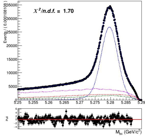
Figure (4.17) Total fit of tagged B^0 mesons on Monte Carlo simulated data.
