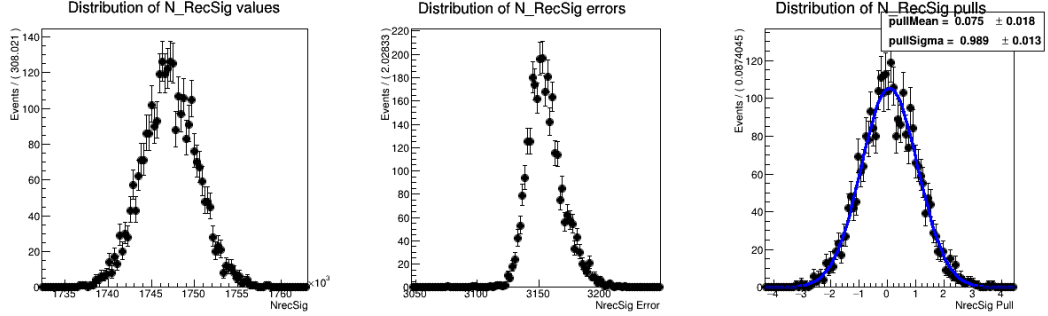
Figure (4.18) Plots showing distributions of the fitted signal yields, errors and the pull distribution of all pseudo-fits.
