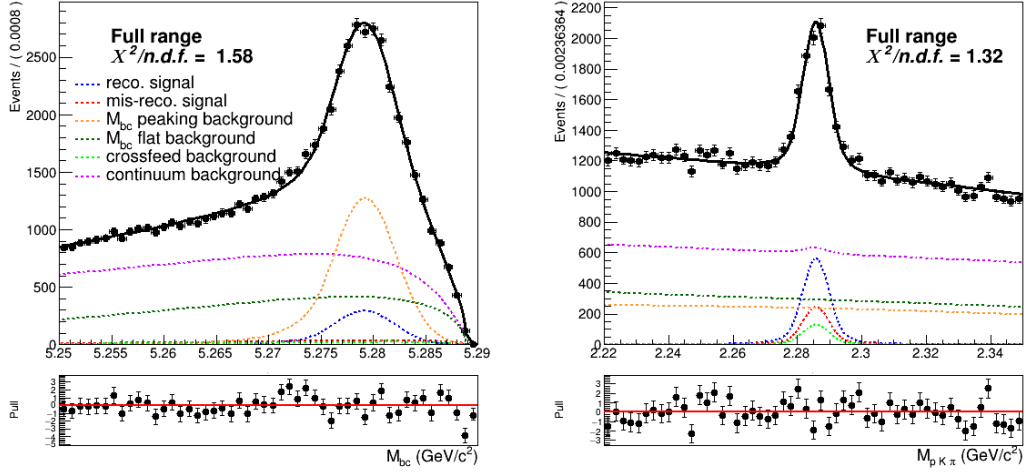
Figure (3.27) Projections of the two dimensional simultaneous fit on stream 0 Monte Carlo simulated data for charged correlated decays.
