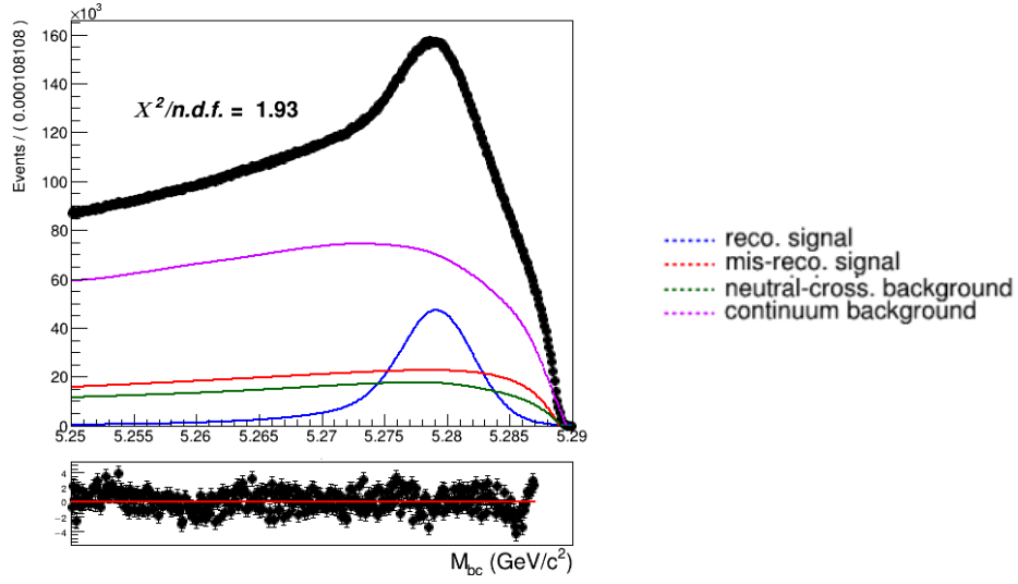
Figure (7.11) Total fit of tagged B mesons
