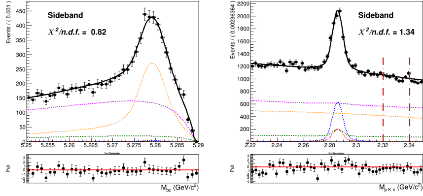
Figure (18) Sideband region of 2.22 < M(pK\pi) < 2.35 \text{ GeV}/c^2 projection of the two dimensional fit on stream 0 Monte Carlo simulated data.
