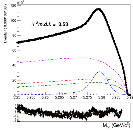
Figure (7.12) Total fit of tagged B^+ mesons candidates on data
