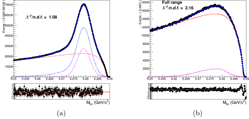
Figure (7.9) On the left: fitted distribution of tagged charged B mesons, reconstructed signal events (magenta) are described by a Crystal Ball whereas the misreconstructed signal events (red) are described by a Novosibirsk function. On the right: Crossfeed distribution fitted with a sum of Novosibirsk (red) and asymmetric Gaussian PDF (magenta)
