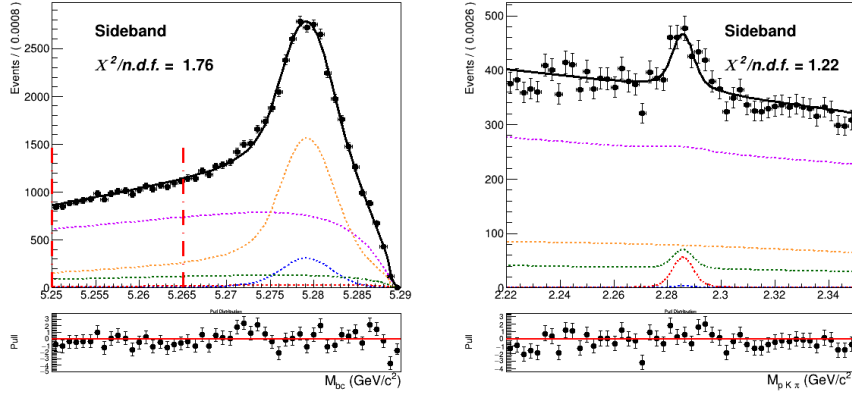
Figure (17) Sideband region of 5.25 < M_{bc} < 5.265 \text{ GeV}/c^2 projection of the two dimensional fit on stream 0 Monte Carlo simulated data.
