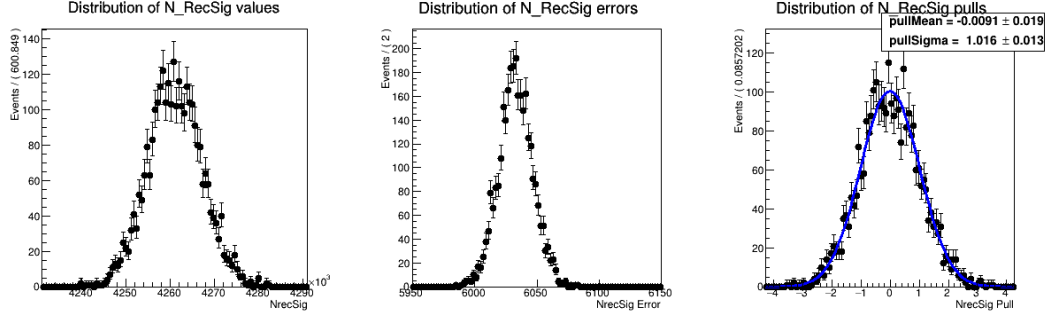
Figure (4.11) Plots showing distributions of the fitted signal yields, errors and the pull distribution of all pseudo-fits. (see Appendix .0.7 for the other free parameters' results)
