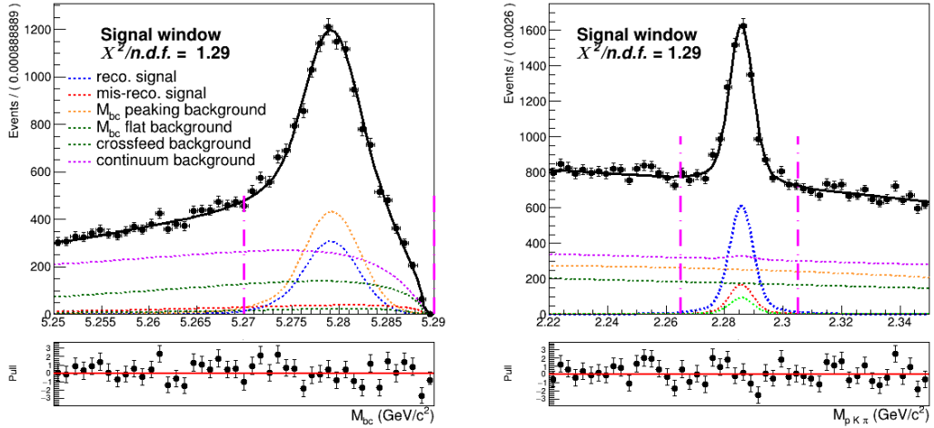
Figure (3.28) Projections of the two dimensional simultaneous fit on stream 0 Monte Carlo simulated data for charged correlated decays (in the signal window)
