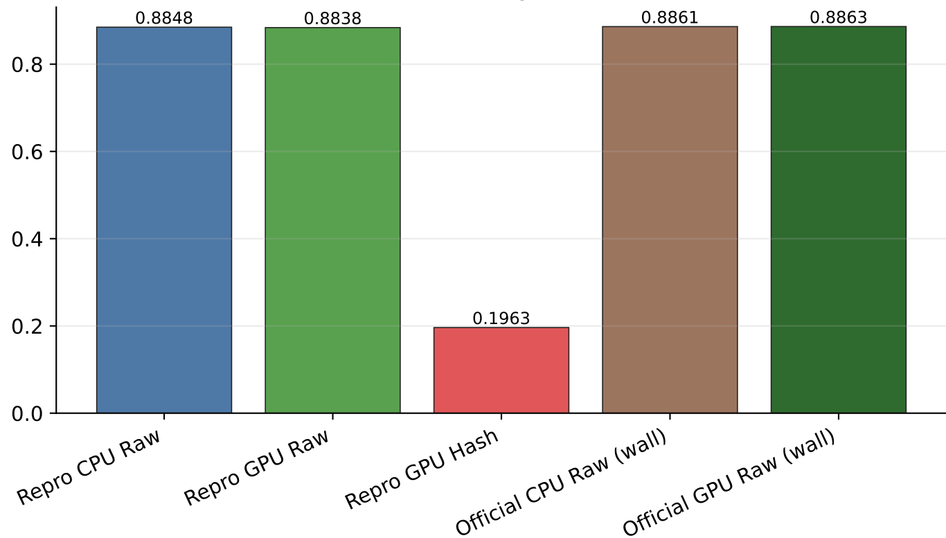
Recall@10
