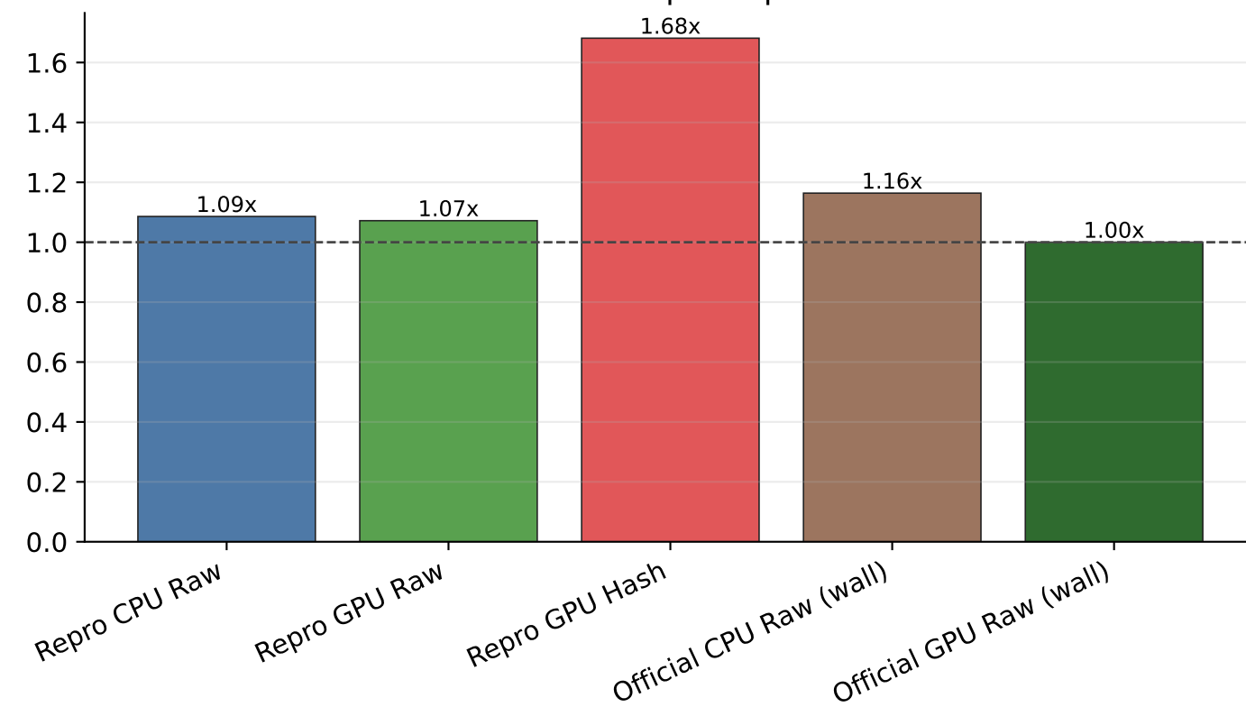
QPS Ratio
