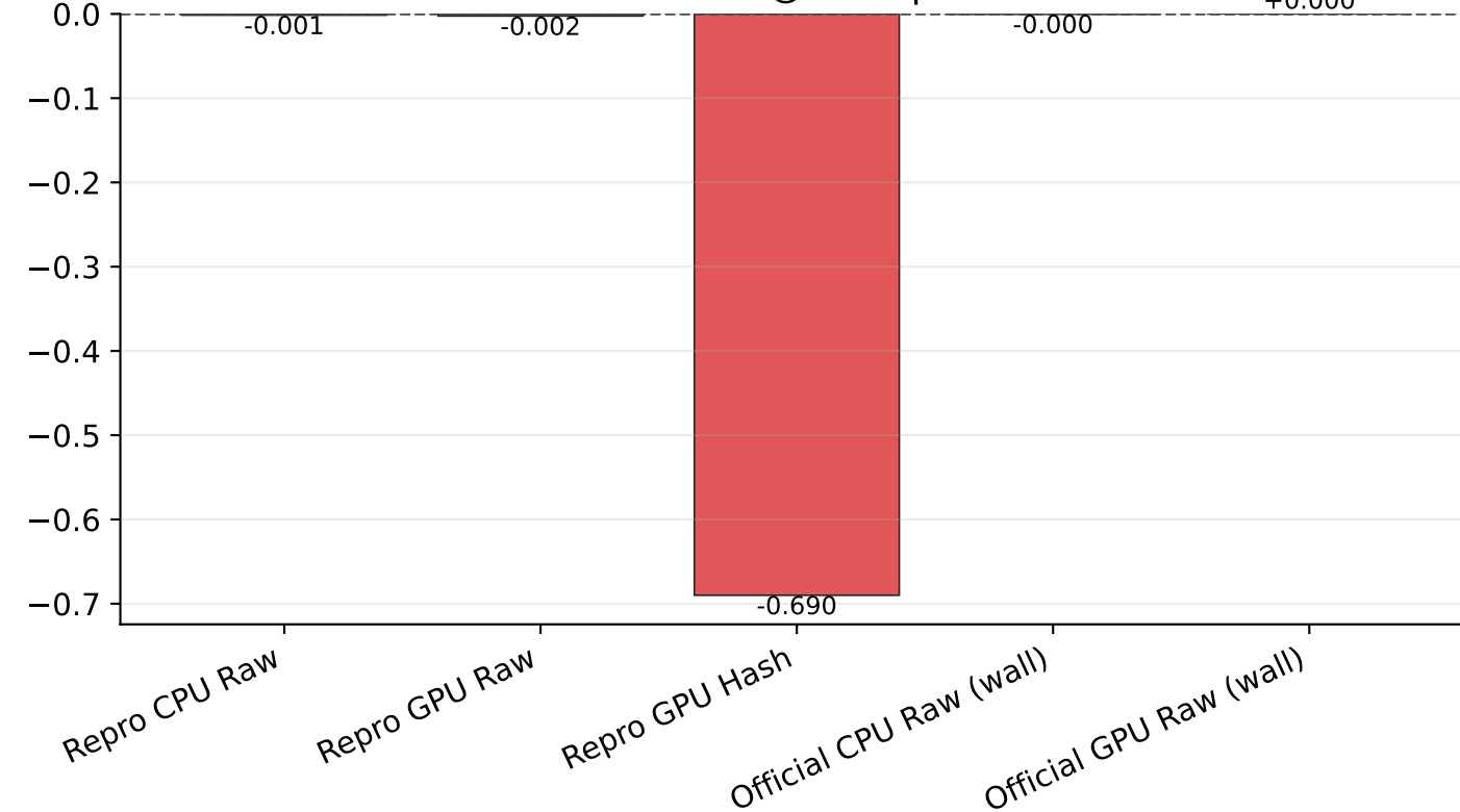
Recall@10 Gap
