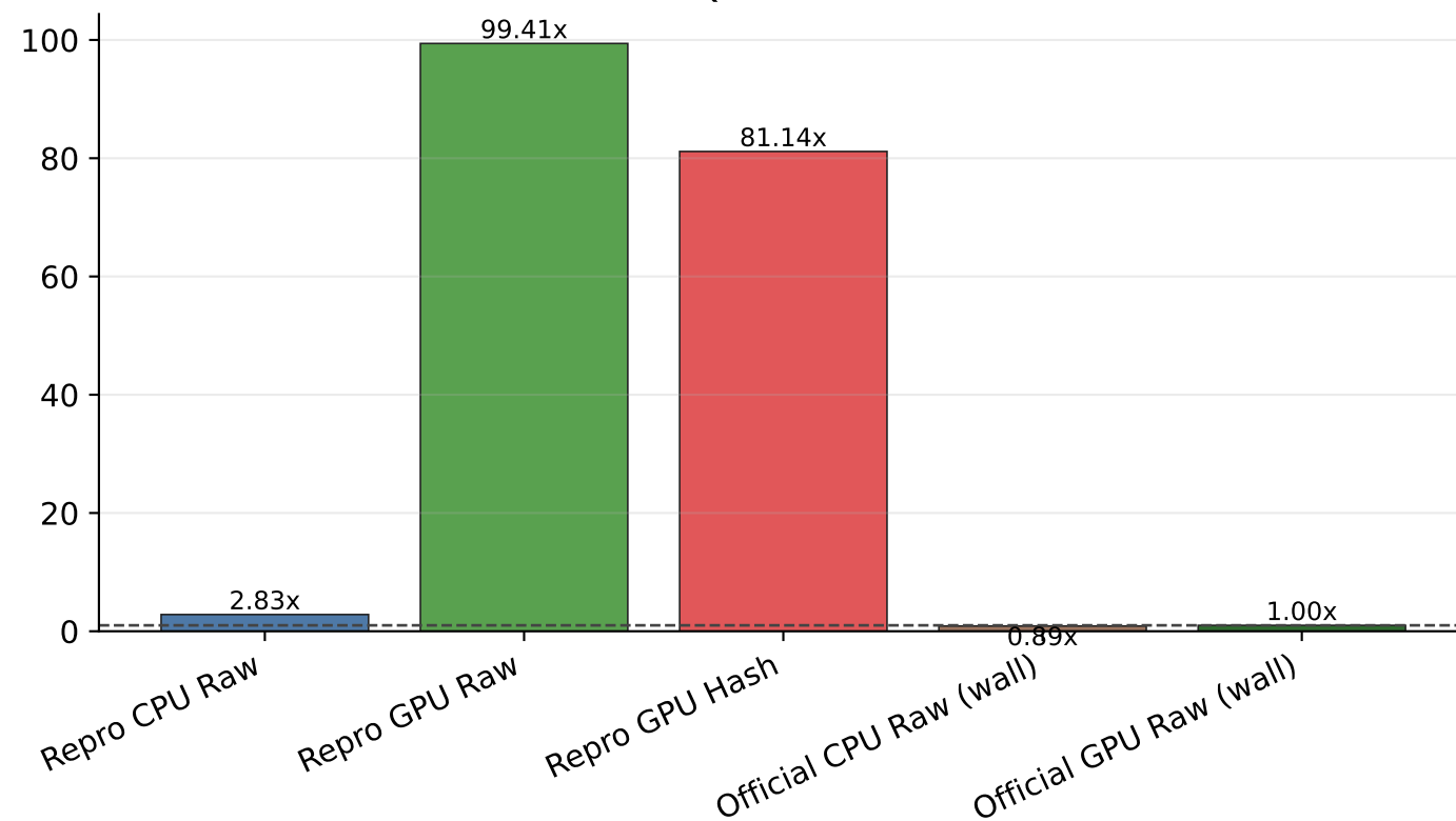
QPS Ratio
