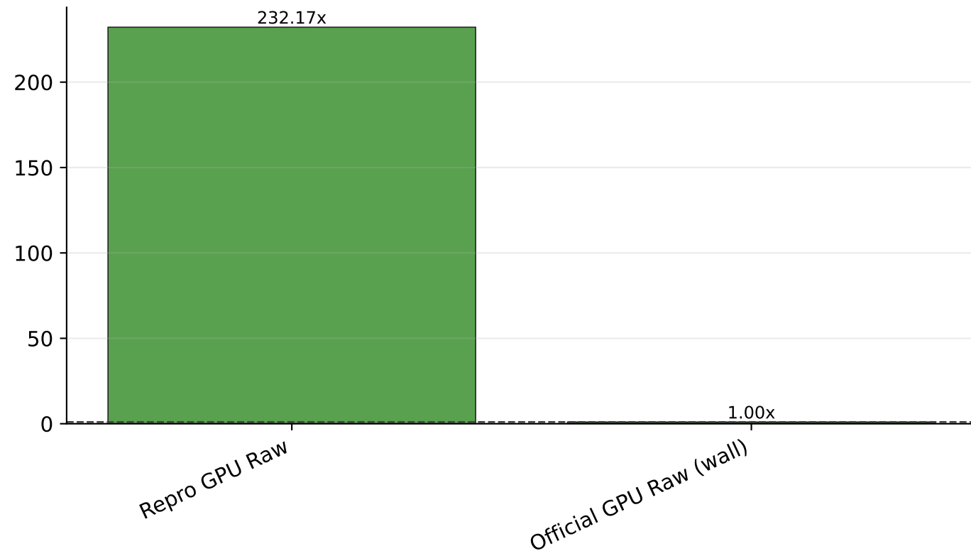
QPS Ratio
