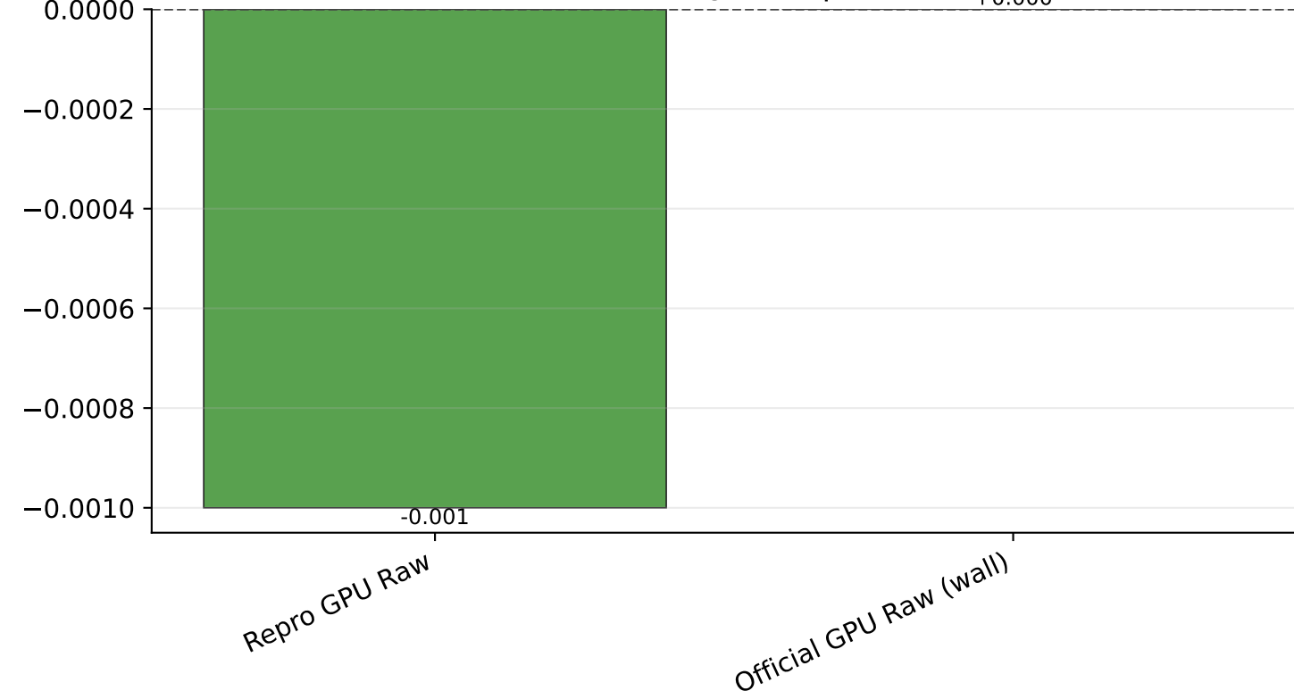
Recall@10 Gap
