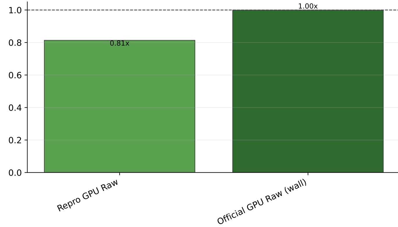
QPS Ratio
