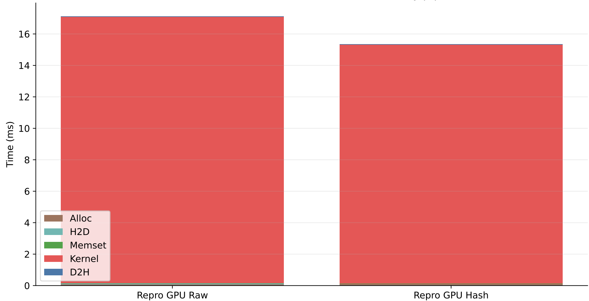
GPU Search Internal Breakdown at Primary pq
